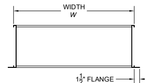
MODEL: ACL645 FRAME: FLANGE FRAME FLANGE-MOUNT (FM)
